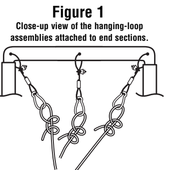
Figure 1 Close-up view of the hanging-loop assemblies attached to end sections.
